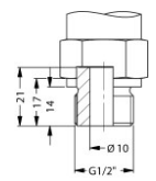
G1/2" open port
